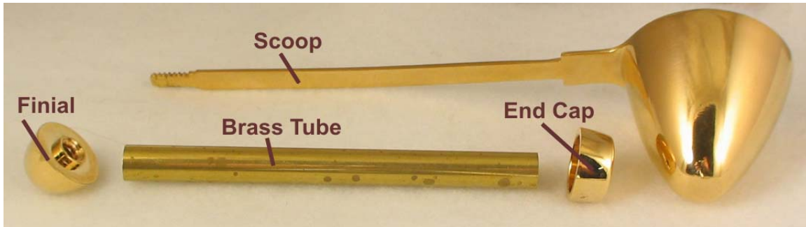
Parts Diagram
