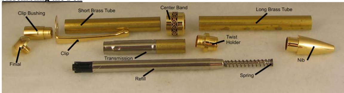
Pen Parts Diagram
