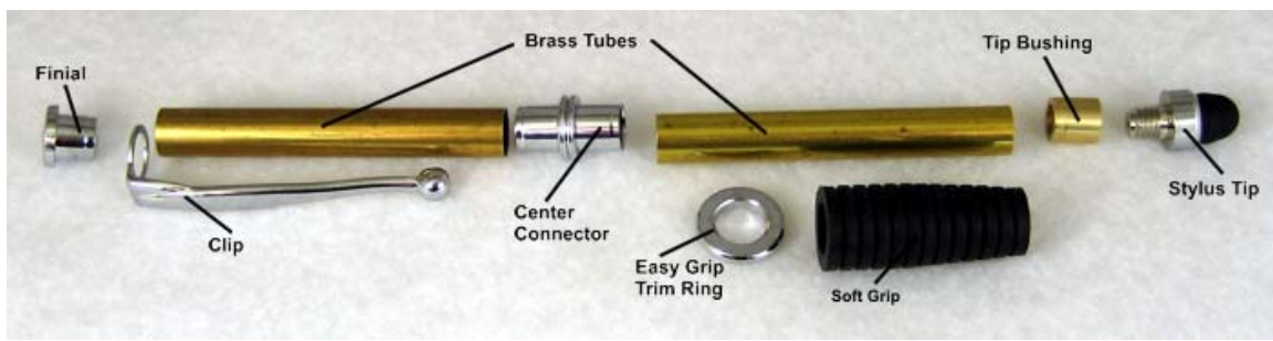
Stylus Parts Diagram
