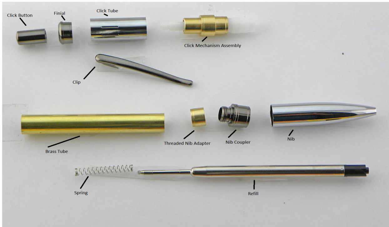
Parts Diagram
